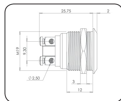
BOPO - PZ bez LED - sans - without - ohne LED
